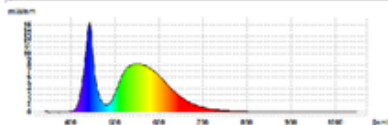
Spectrum
